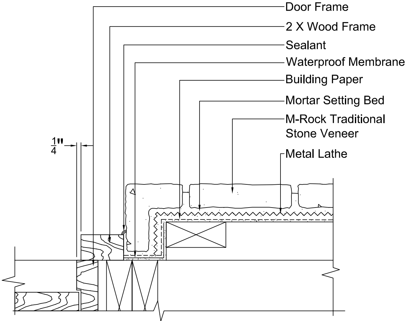
Door Jamb Corner Return Detail M-Rock Stone Manufacturing
