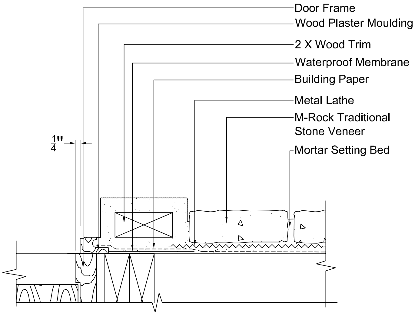
Door Jamb Furred Trim Detail M-Rock Stone Manufacturing
