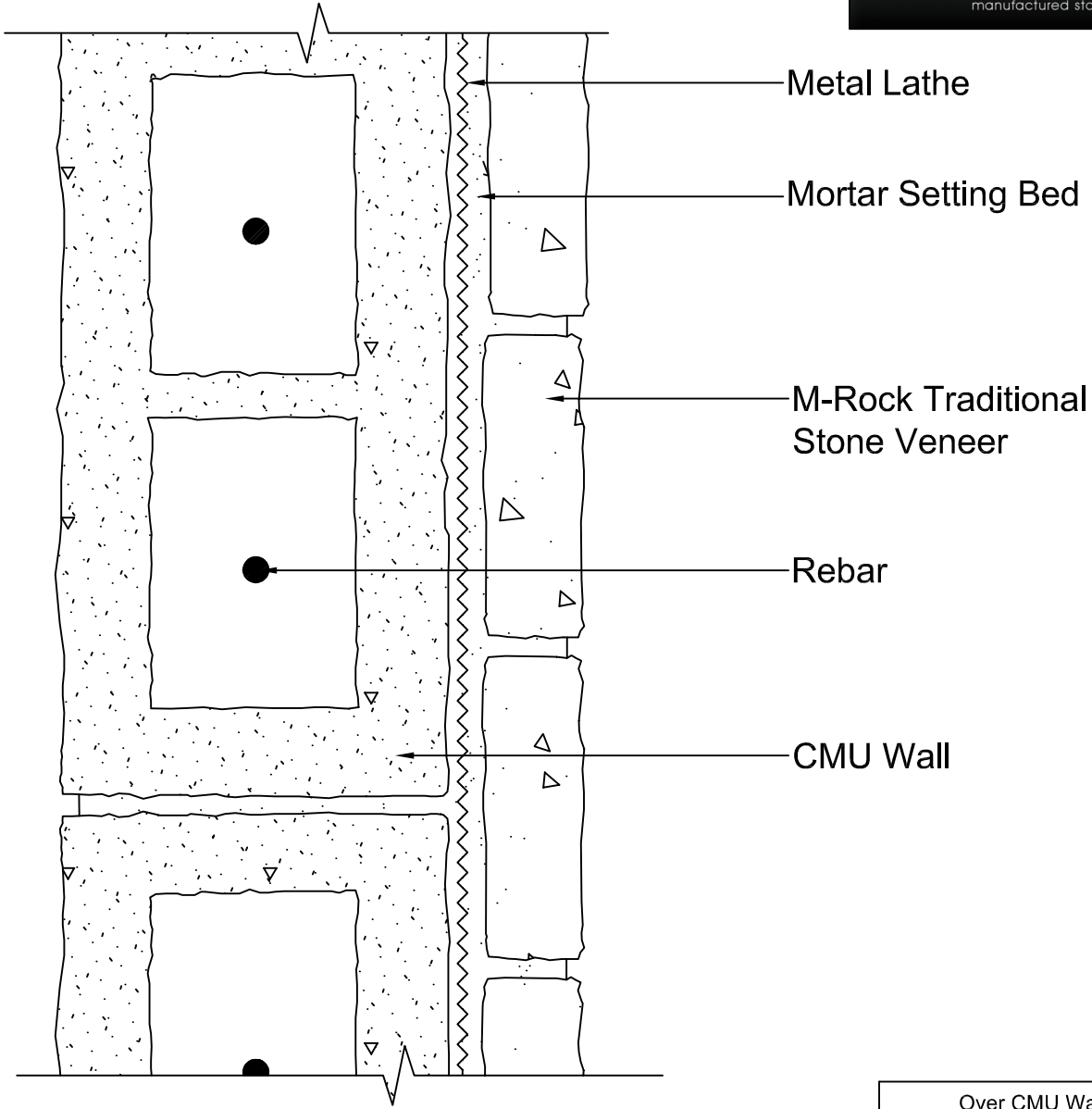
Over CMU Wall Detail M-Rock Stone Manufacturing
