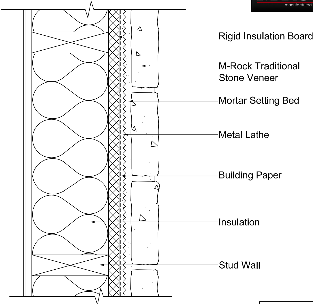
Over Rigid Insulation Detail M-Rock Stone Manufacturing
