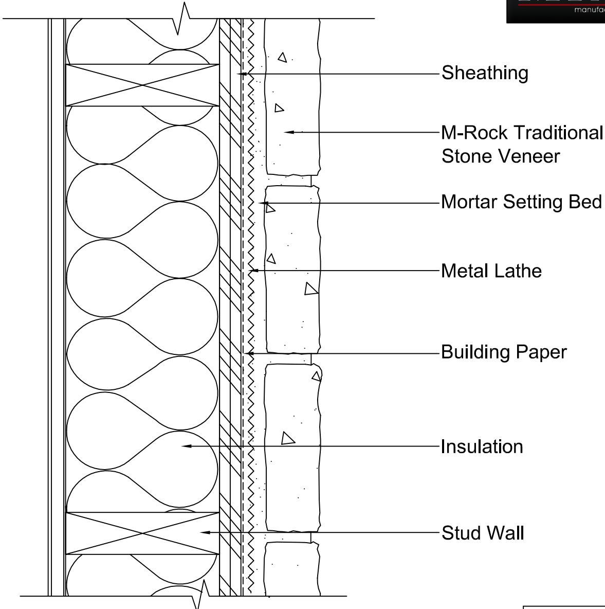
Over Sheathing Detail M-Rock Stone Manufacturing
