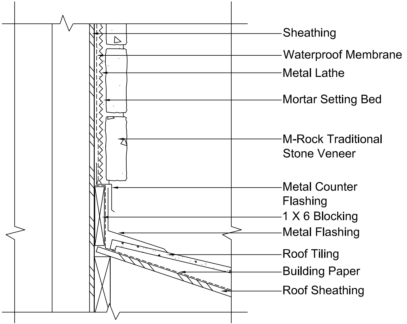
Transition Roof to Wall Detail M-Rock Stone Manufacturing
