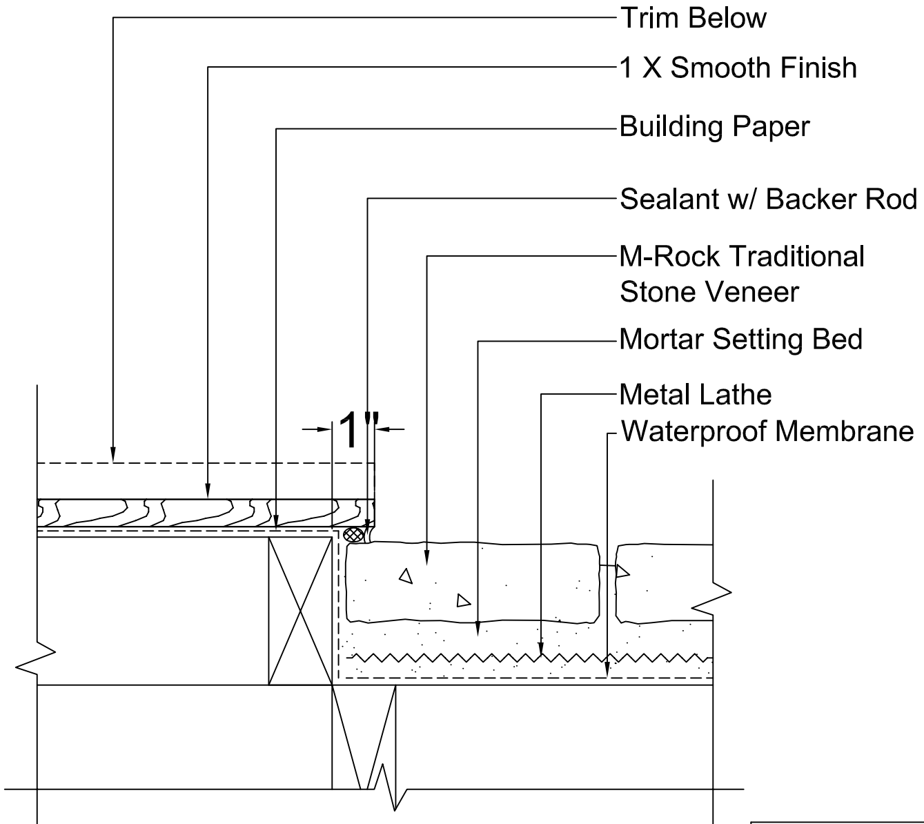
Transition Stone Siding Detail M-Rock Stone Manufacturing
