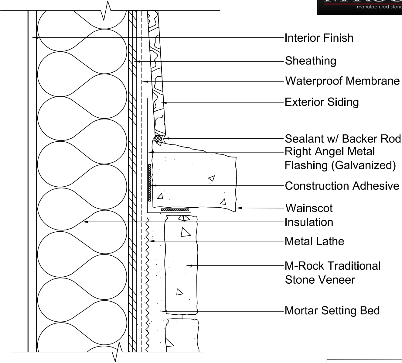
Wainscot Installation Detail M-Rock Stone Manufacturing
