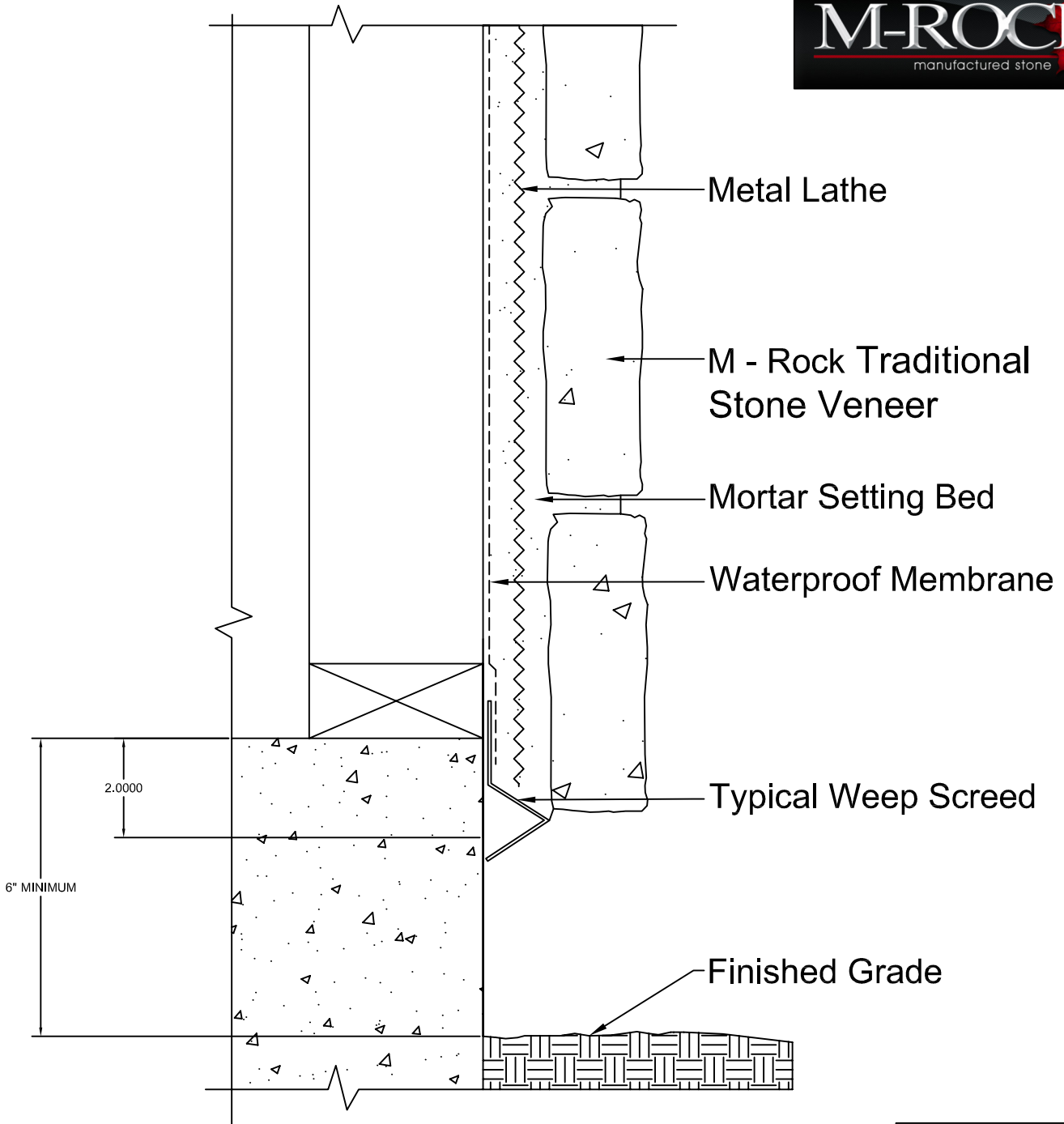
Weep Screed Detail M-Rock Stone Manufacturing
