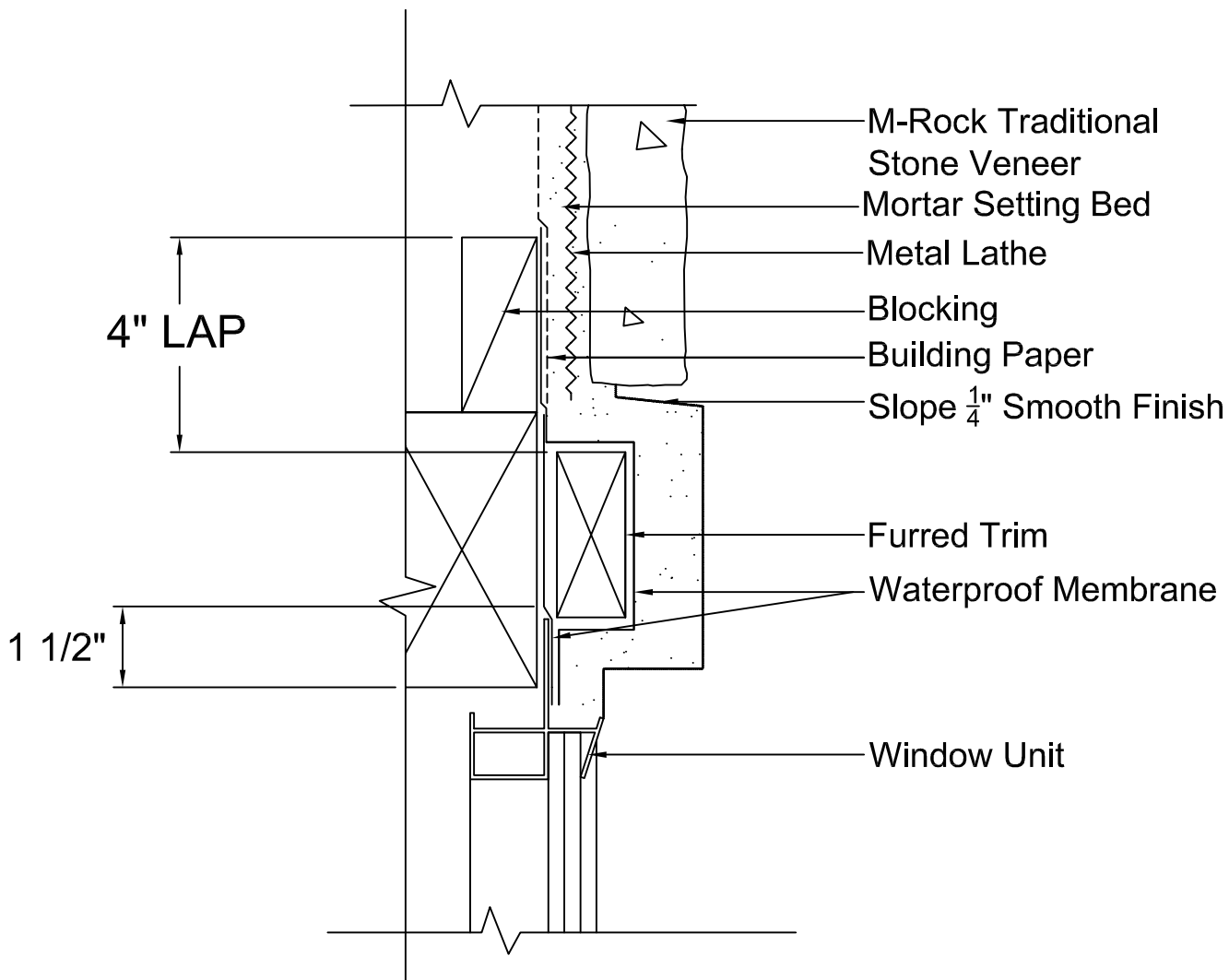
Window Header Furred Trim Detail M-Rock Stone Manufacturing
