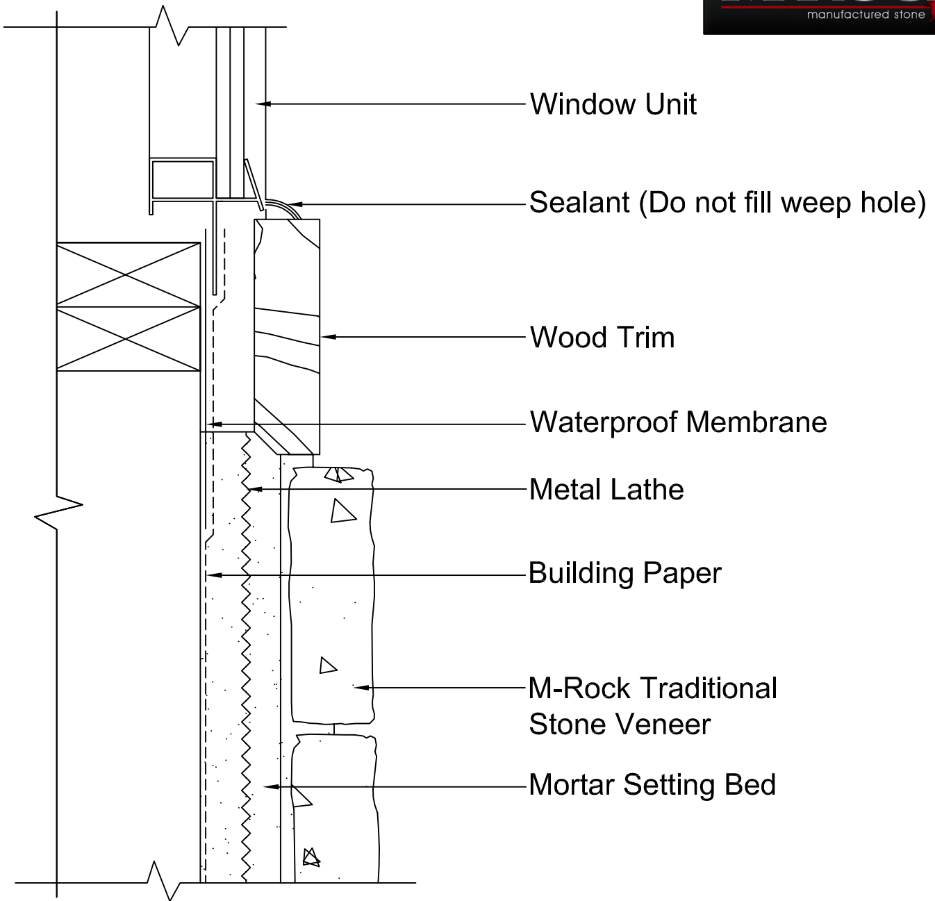
Window Sill Wood Trim Detail M-Rock Stone Manufacturing
